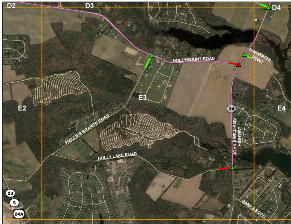
Figure 49. AM Level of Service (Grid E3)
