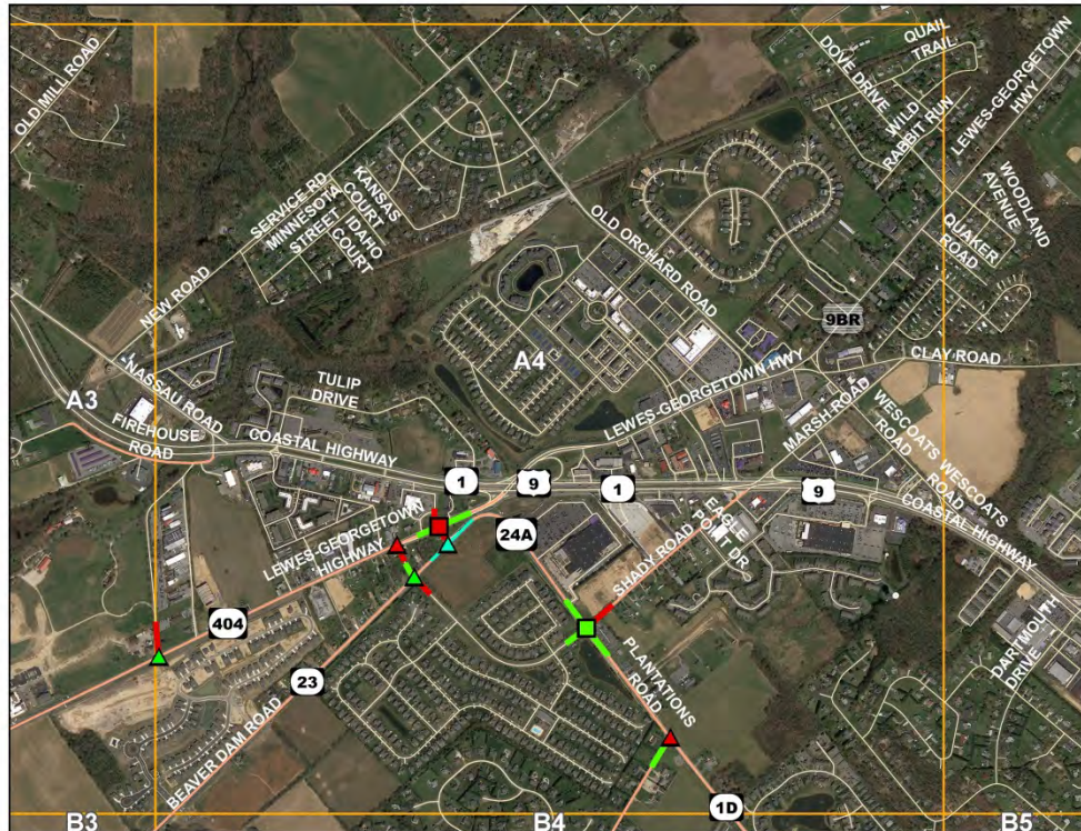
Figure 15. AM Level of Service (Grid A4)
